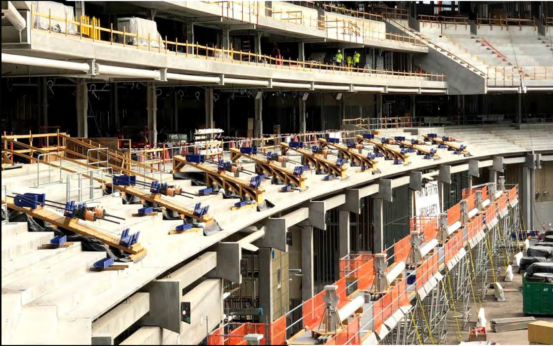
Above and Below: Freyssinet cablenet prep work continues to progress in the bowl.
